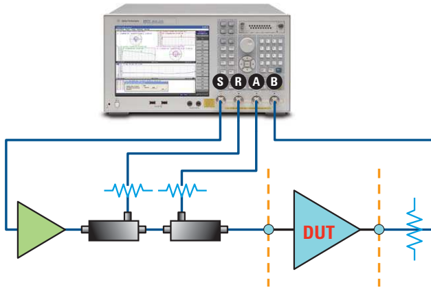
High-power measurement using external test set mode
